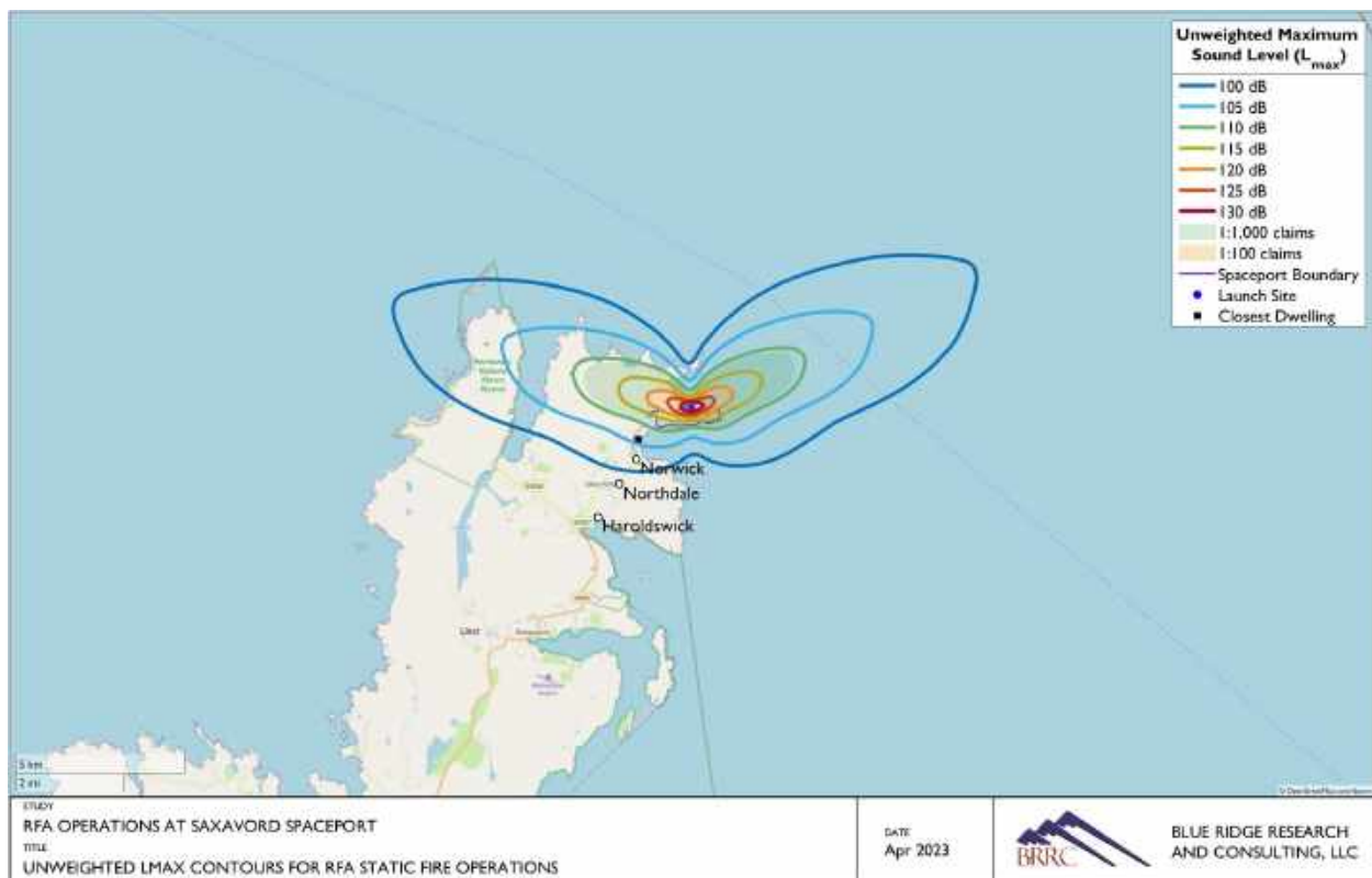
Figure 6. Unweighted maximum sound level contours for RFA ONE static fire operations.
