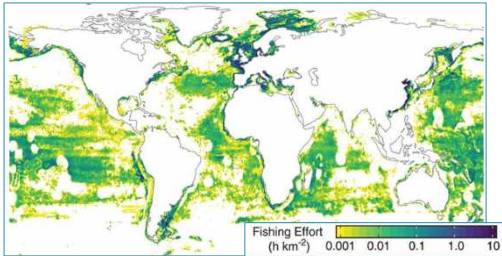
Figure A10.8: Total global fishing effort [hours fished per square kilometre ( \text{h/km}^2 )] in 2016 by all vessels with automatic identification system enabled (From: Kroodsmma et al., 2018)
