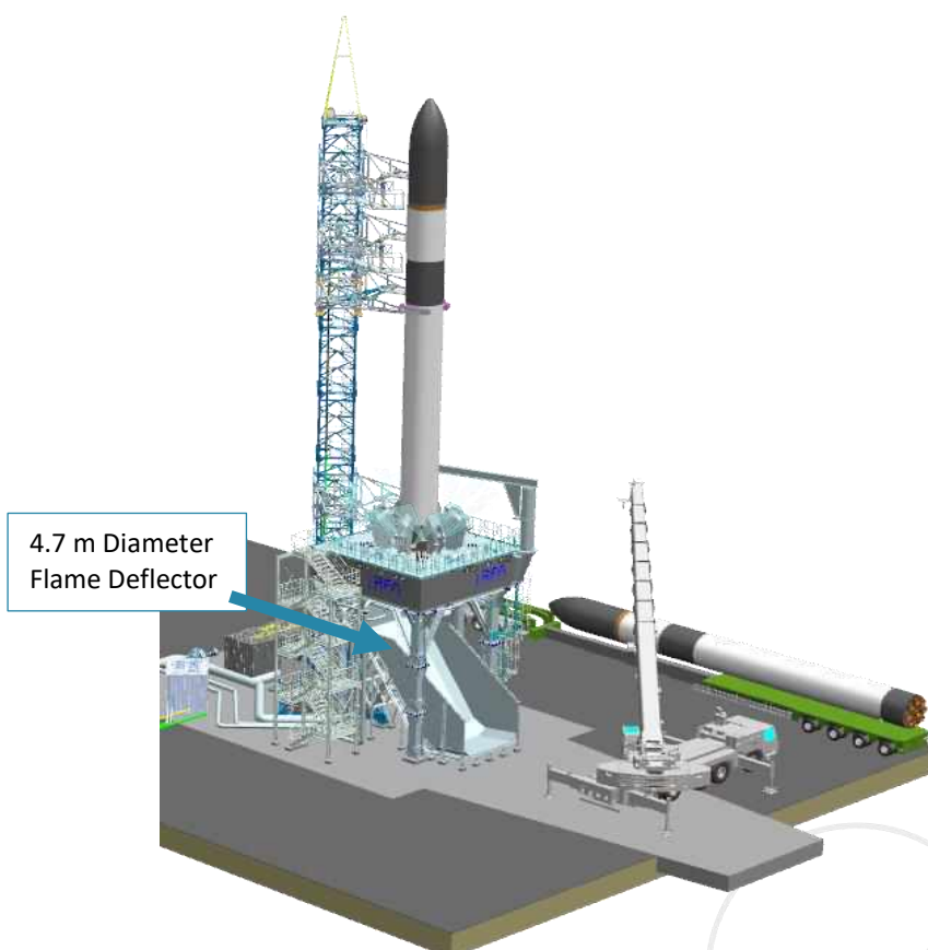
Figure 1 Schematic of Launch Rig
